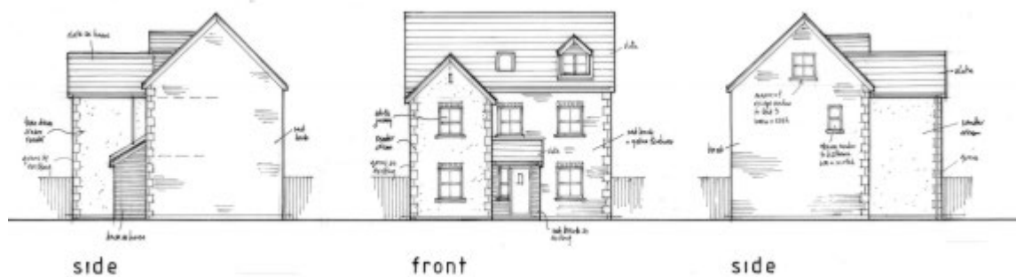
Fig. 1.3 Proposed Elevations
