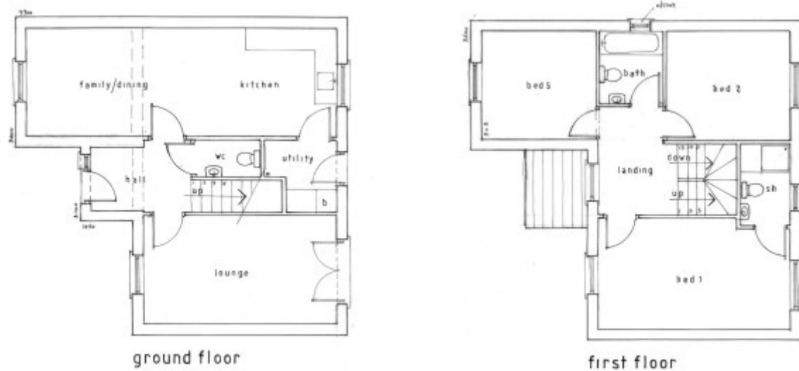
Fig. 1.2 Proposed Floor Plans
