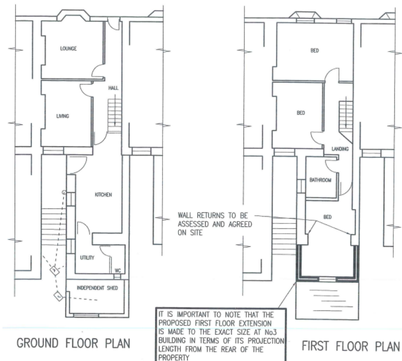
Fig. 1.3 Proposed Floor Plans
